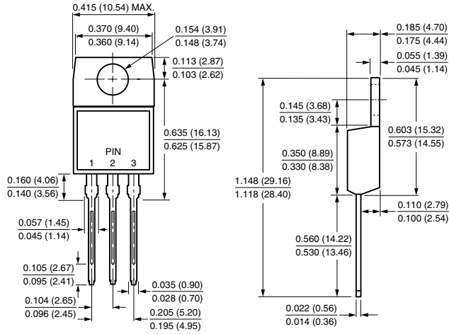
TO-262AA
